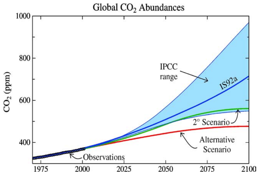
Figure 15. CO 2 in the range of IPCC (2001) “marker” scenarios, and in our “alternative” and “2° C” scenarios. In the alternative scenario \Delta CO 2 decreases linearly from 1.7 ppm/year in 2000 to 1.3 ppm/year in 2050 and then linearly to zero in 2100; CO 2 peaks at ~475 ppm in 2100. In the “2°C” scenario \Delta CO 2 increases linearly from 1.7 ppm/year in 2000 to 3 ppm/yr in 2050 and then decreases linearly to zero in 2100; CO 2 peaks at ~560 ppm in 2100. Upper and lower limits of IPCC range are their scenarios A1FI and B1 [IPCC, 2001, Appendix II, p. 807 and Figure 18, p.65]. IS92a is the updated version of that scenario in IPCC (2001), which incorporates recent carbon cycle modeling. A still broader range of IPCC scenarios is included in their Special Report on Emission Scenarios (SRES) document (Reference 12b). CO 2 scenarios for the alternative and “2°C” scenarios are given at http://www.giss.nasa.gov/data/simodel/ghgases/fig1A.ext.txt .
