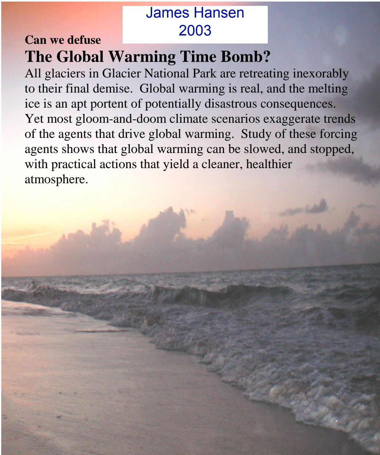
Figure 1. Wind and tides mix the ocean to great depths. Thus, because of the thermal inertia of this ocean water, it requires at least several decades for the ocean temperature to respond fully to a climate forcing.
